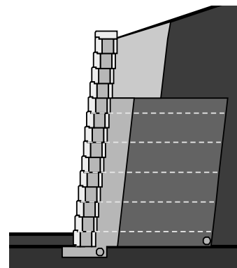
No-fines concrete in the Upper Structure cannot be less than the standard minimum of 2 ft (60 cm) and is commonly designed to be 40% of the Upper Structure height
