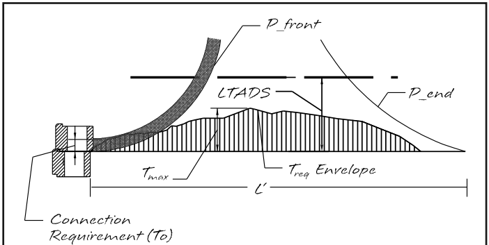
Figure 8-12. Geogrid Pullout Envelope
