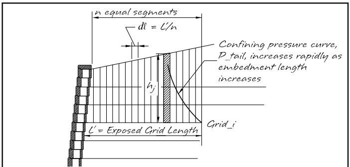
Figure 8-13. Geogrid Pullout Confining Pressure
