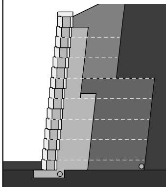
Geogrid lengths in the Upper Structure cannot be less than the standard minimum of 4 ft (120 cm) or 60% of the Upper Structure height
